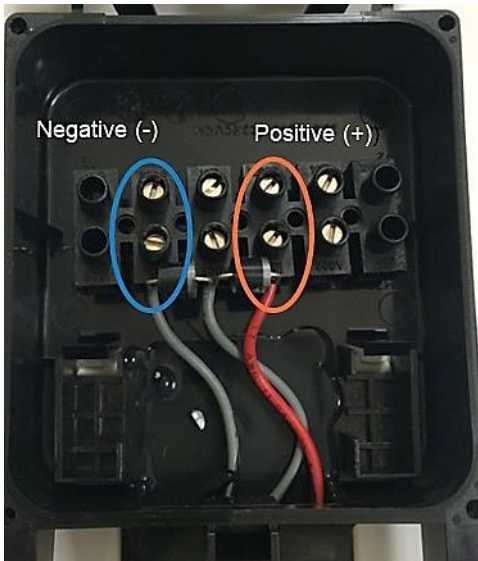
Figure 29: Power Cable Connection to Solar Cell Terminals.
