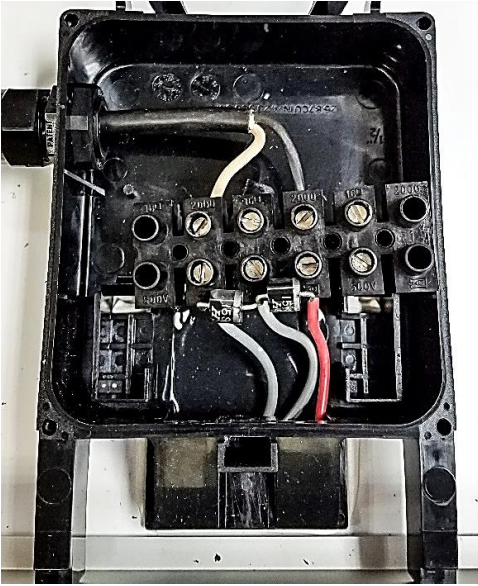
Figure 30: Attach Power Cable to Screw Terminals
