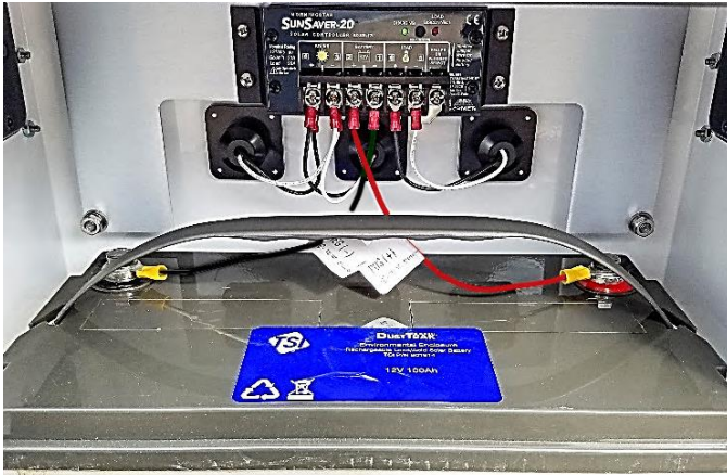
Figure 27: Install the Solar Battery and Connect to Controller
