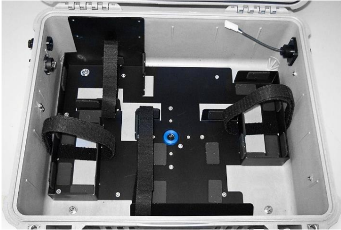
Figure 16: DustTrak™ Aerosol Monitor VELCRO® Straps
