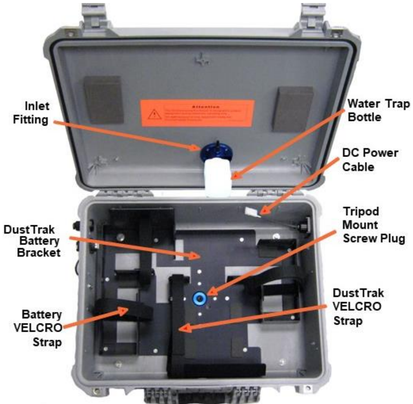
Figure 1: Inside View of Environmental Enclosure
