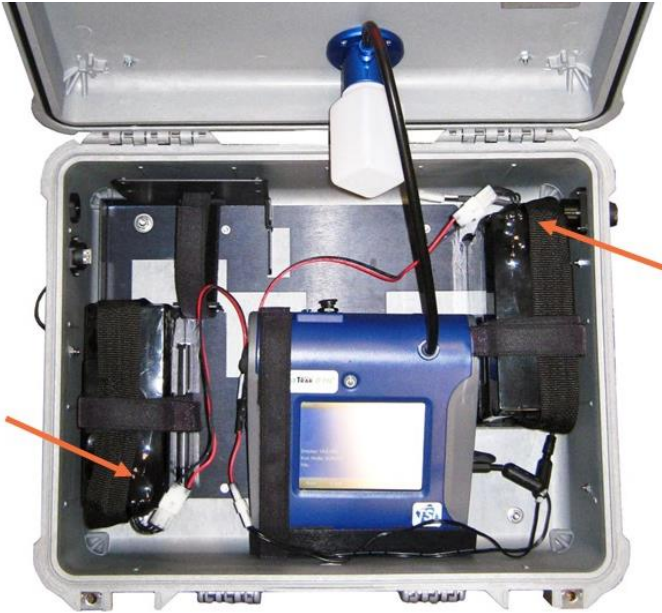
Figure 12: Install the Dual Battery Pack System
