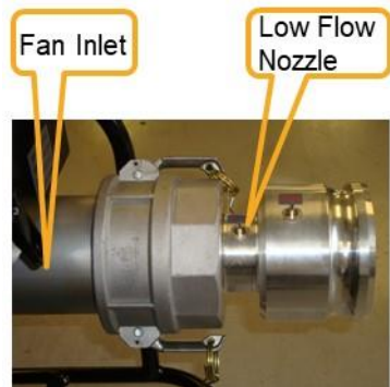
Figure 7. Positive Pressure, Low-Flow Setup
